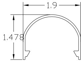
A2 TOP RAIL
