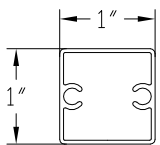
A9 1" PICKET
