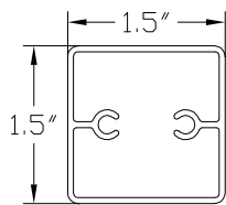
A10 1.5" PICKET
