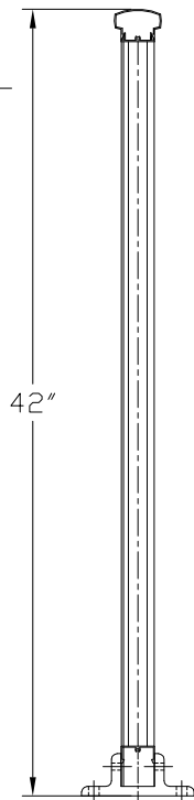
A2 TOP RAIL
