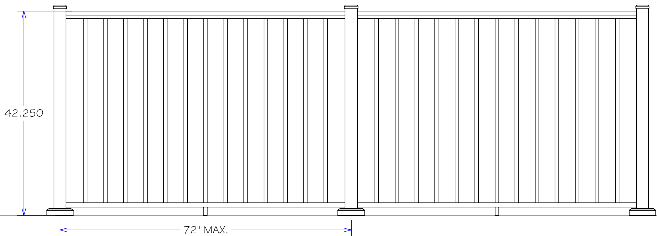
200 RAILING ELEVATION
