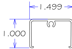
A201 TOP/BOTTOM RAIL
